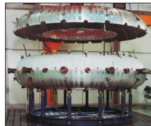
RFX vacuum vessel
