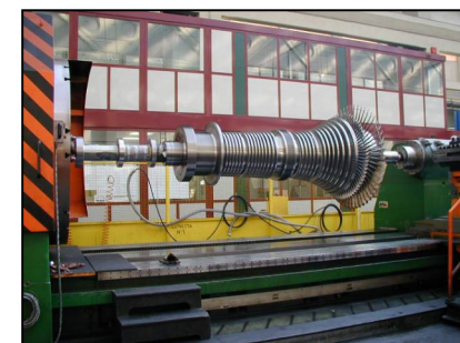
Steam turbine and axial compressor rotors (forged, machined and assembled)
