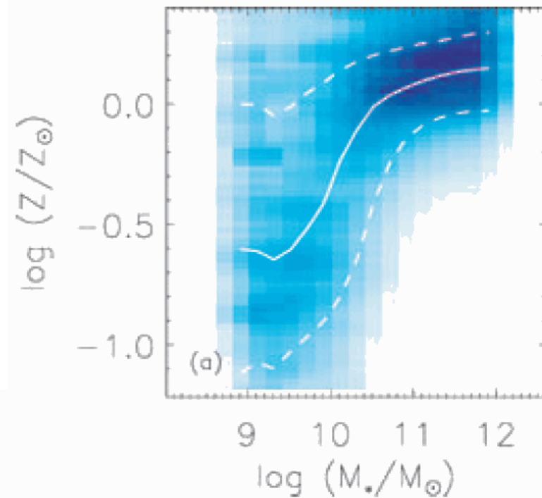
Stellar metallicity SDSS galaxies Gallazzi+05
